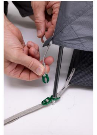
Hold Fast Clips and Adjustable Peg Loops
